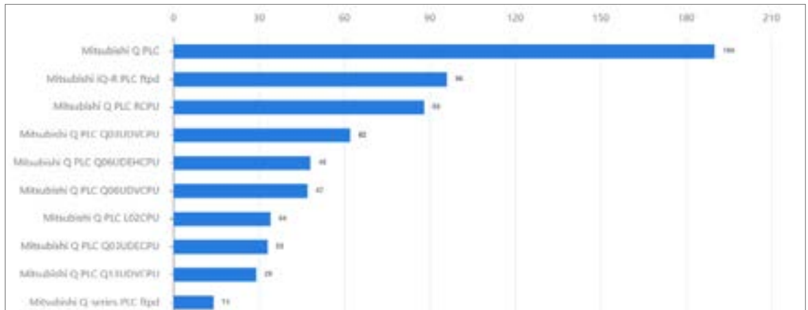
Figure 6: Internet exposure of Mitsubishi Q-PLC range
